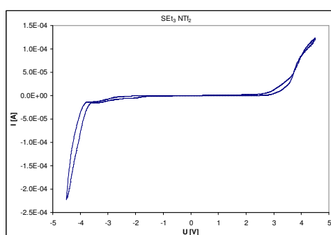
Cyclovoltammogram of \text{SEt}_3 \text{NTf}_2 .
